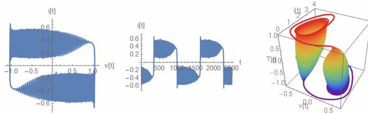
2D phase portrait, time domain waveform, and a 3D phase portrait
